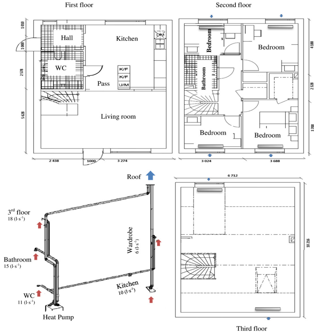
Fig. 3. Floor plan showing the location of ventilation radiators in second and third floors and the ventilation system (values are in mm and plan is not to scale).
