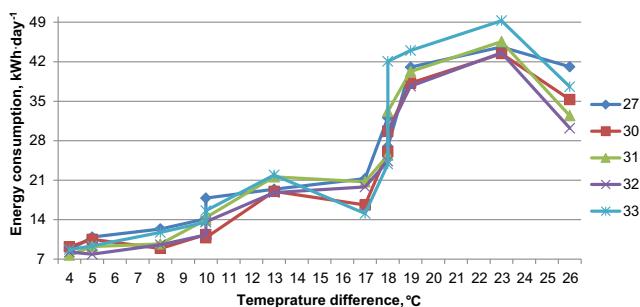
Fig. 8. Heating load as a function of temperature difference between inside and outside for the five dwellings.
