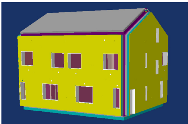
Fig. 5. Simulation of a pair of semi-detached houses using IDA ICE 4 software.
