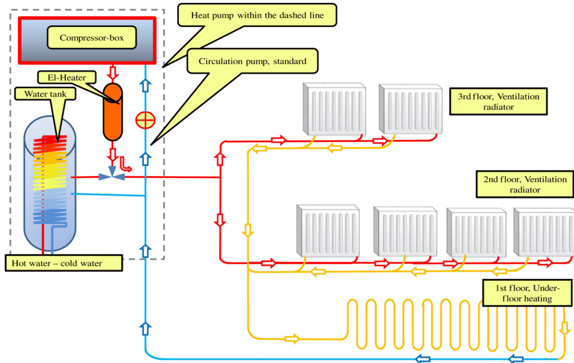
Fig. 4. Low temperature hydronic heating system connected to the heat pump.
