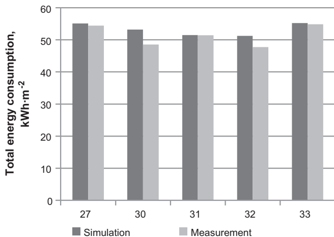
Fig. 10. Comparison of total consumption between measurement and simulation in the five houses studied.
