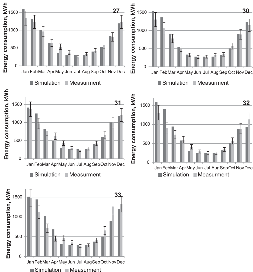
Fig. 9. Comparison of measured and calculated energy consumption in the five houses studied.
