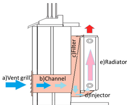
Fig. 1. Main parts of a ventilation radiator: (a) Vent grill on the external wall, (b) Channel through wall, (c) Filter, (d) Injector or inlet (with or without mixing of cold supply air with room air), (e) Traditional radiator [9].
